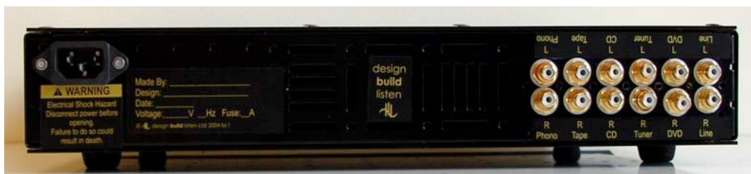
ezChassis as a Preamp. 'Upside-down" with IEC mains socket. Label covers 'speaker' holes
